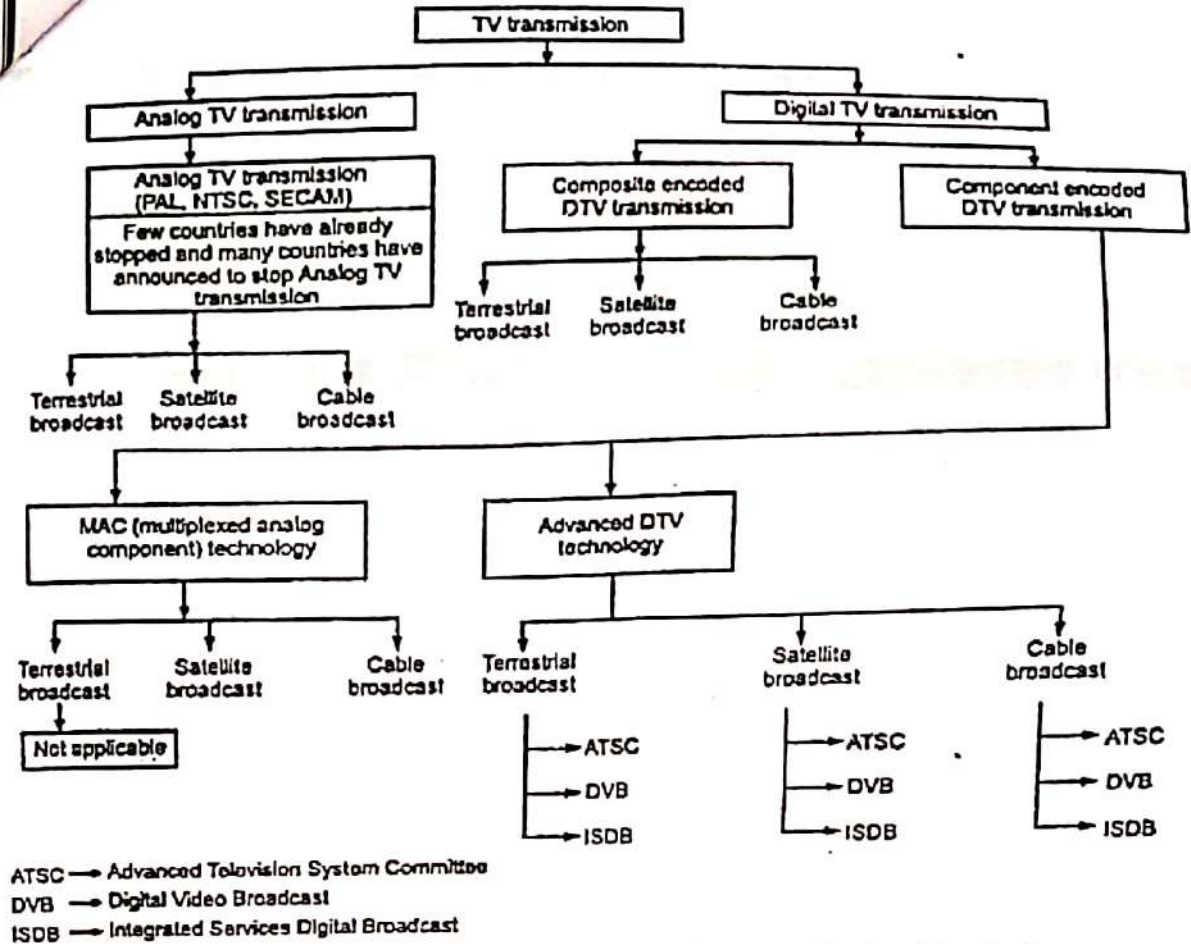
Figure 1:- Analog and Digital TV signal transmission Techniques
